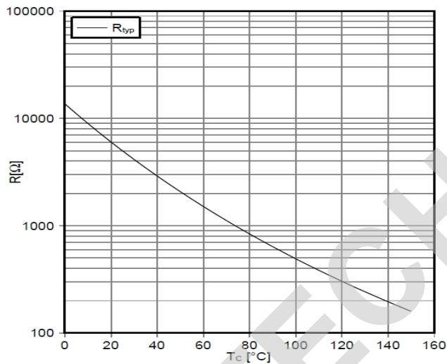
Fig.15 NTC-Thermistor-temperature characteristic
