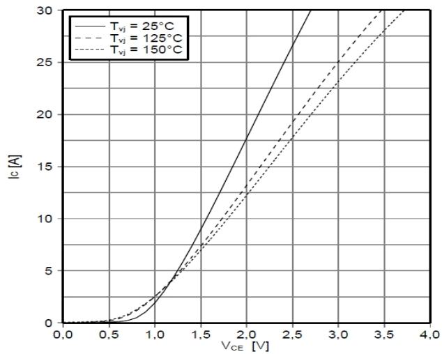
Fig.13 output characteristic IGBT, Brake-Chopper
