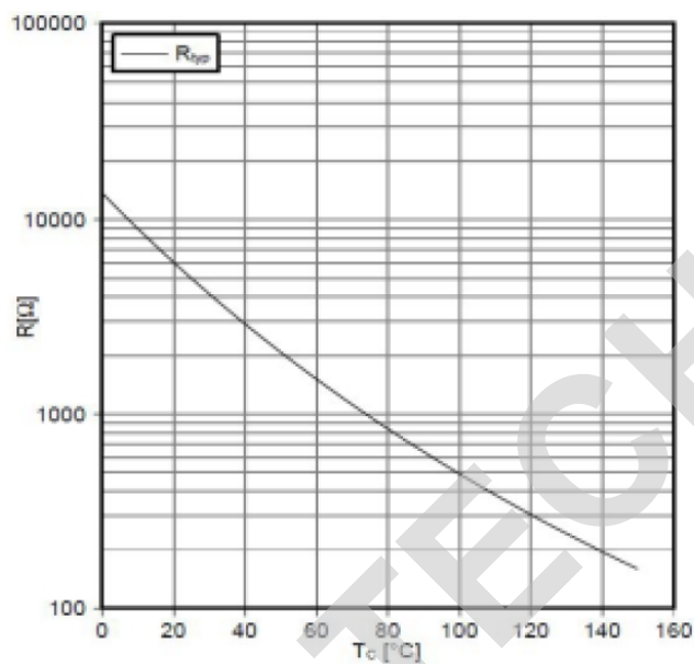
Figure11. NTC-Thermistor-temperature characteristic
