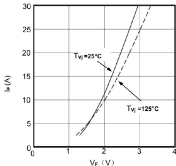
Figure7. Diode Forward Characteristics
