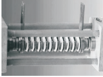
Fig.4 30KV RSD STACK
